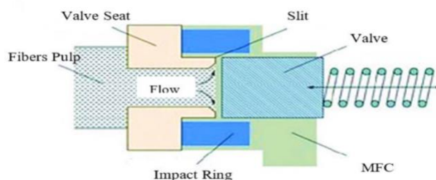
Figure 6. Piston gap homogenizer [35].
