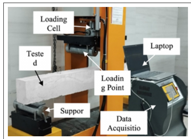
Figure 4. Test setup.
