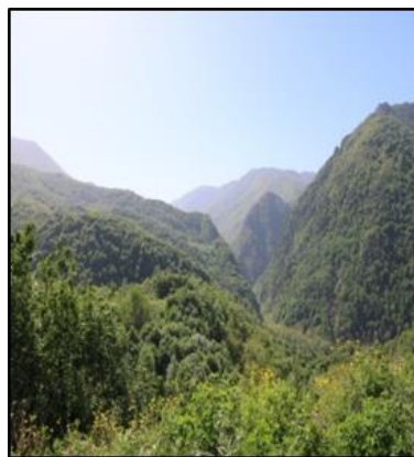
Figure 4. General view of Samanlı Mountains
