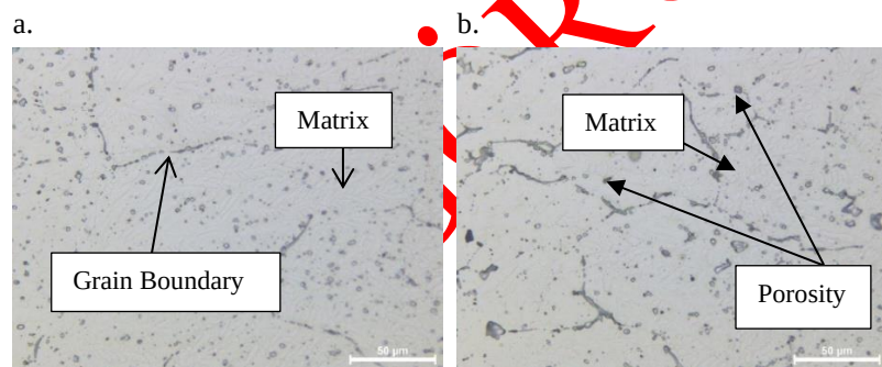
Figure 6. Optical microscope image of the sample of the 2nd wall at 20x magnification
