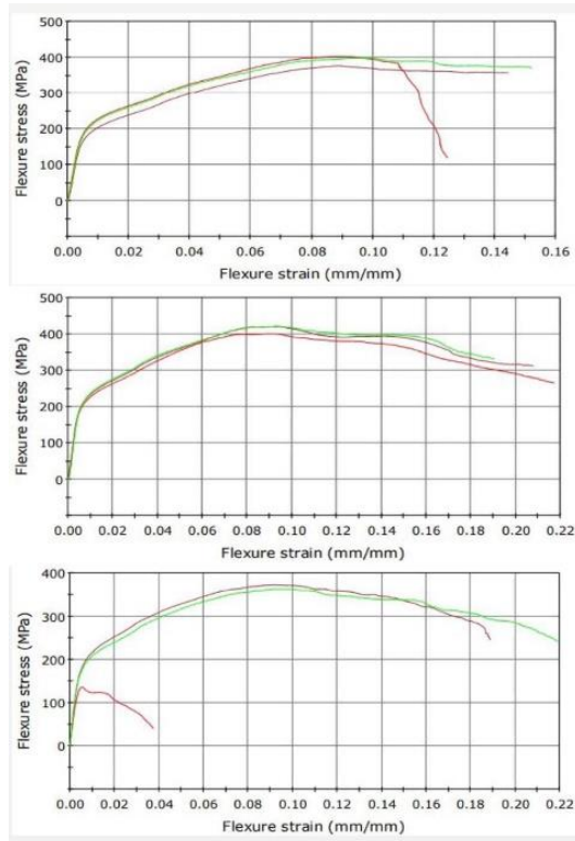
Graphic 3. Flexural Stress–Strain Curves for Walls 1, 2, and 3, respectively
