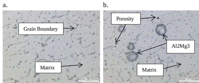
Figure 5. Optical microscope image of the sample of the 1st wall at 20x magnification
