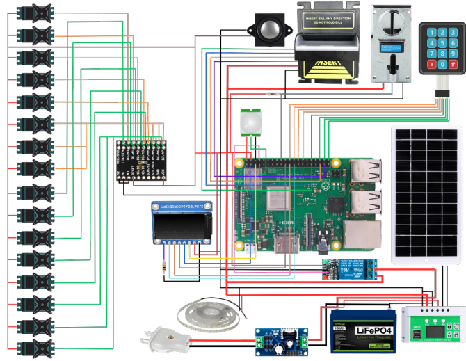
Fig. 3: System Architecture
