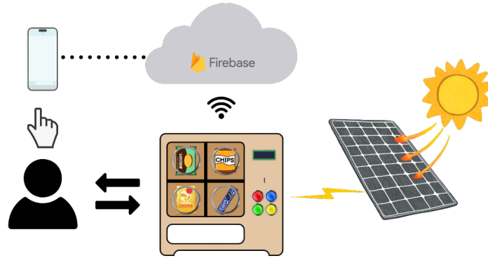
Fig. 2: Conceptual Framework.
