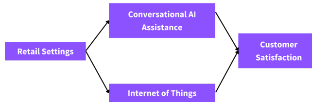
Fig. 1: Theoretical Framework.
