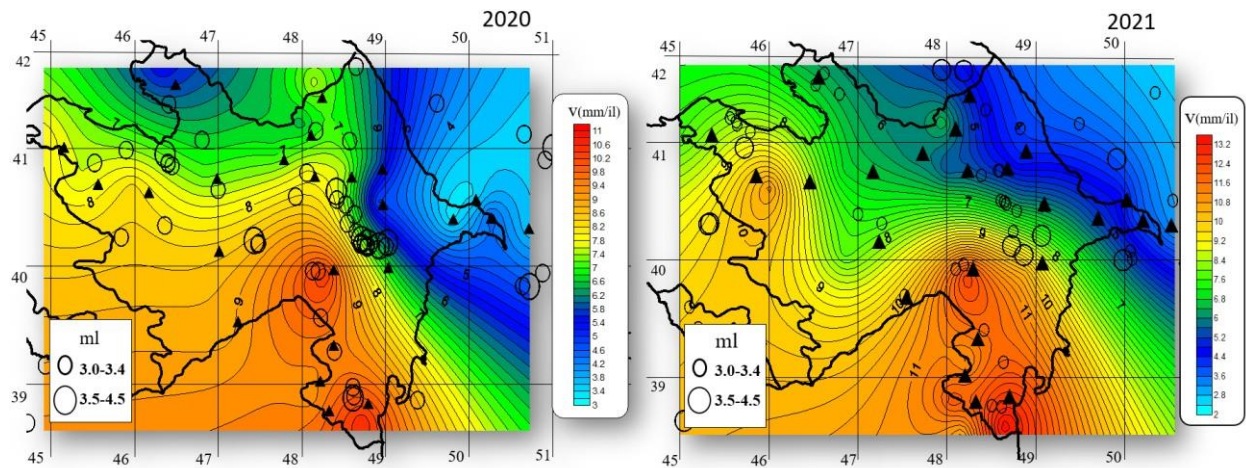
Fig. 2. Scheme of the spatial distribution of velocities according to GPS station data for 2020-2021
