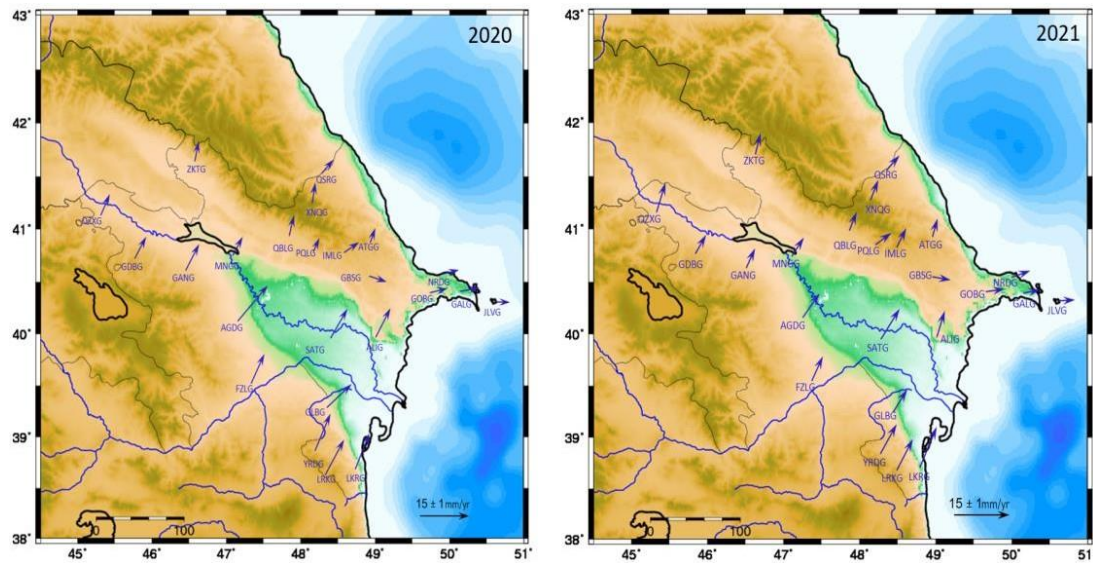
Fig. 3. GPS horizontal velocity vectors for 2020-2021
