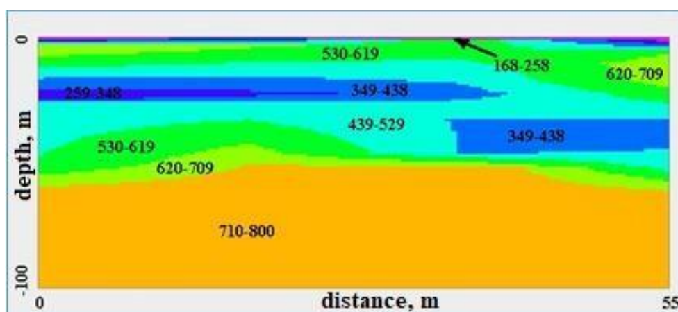
Fig. 11. 2D shear wave velocity section on seismic profile № 3
