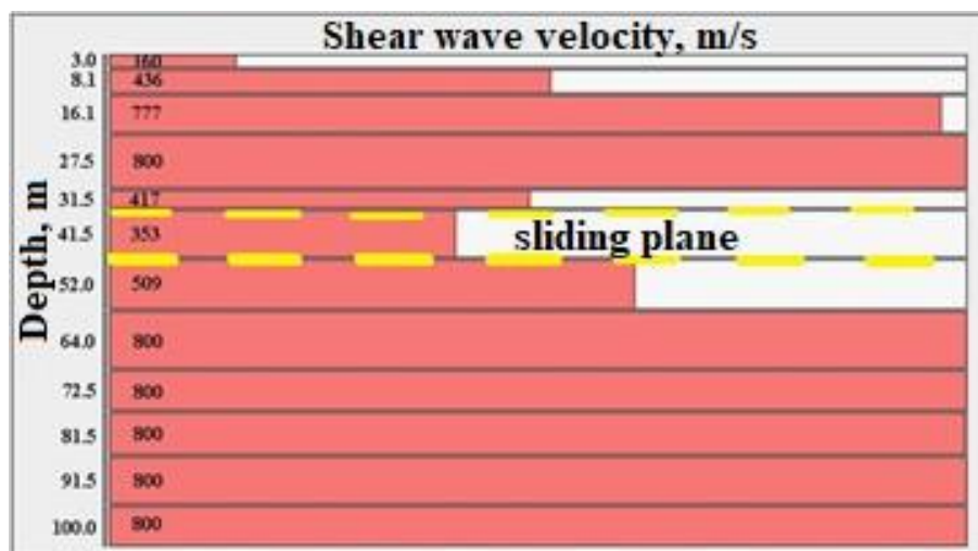
Fig. 10. 1D shear wave velocity section on seismic profile № 1
