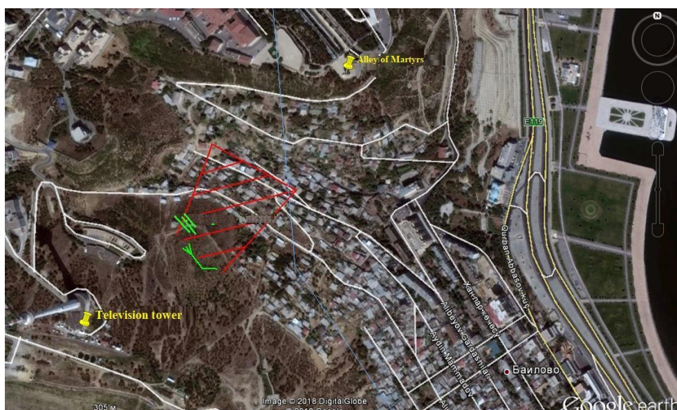
Fig. 1. General view of the landslide with observed main fractures in the area
