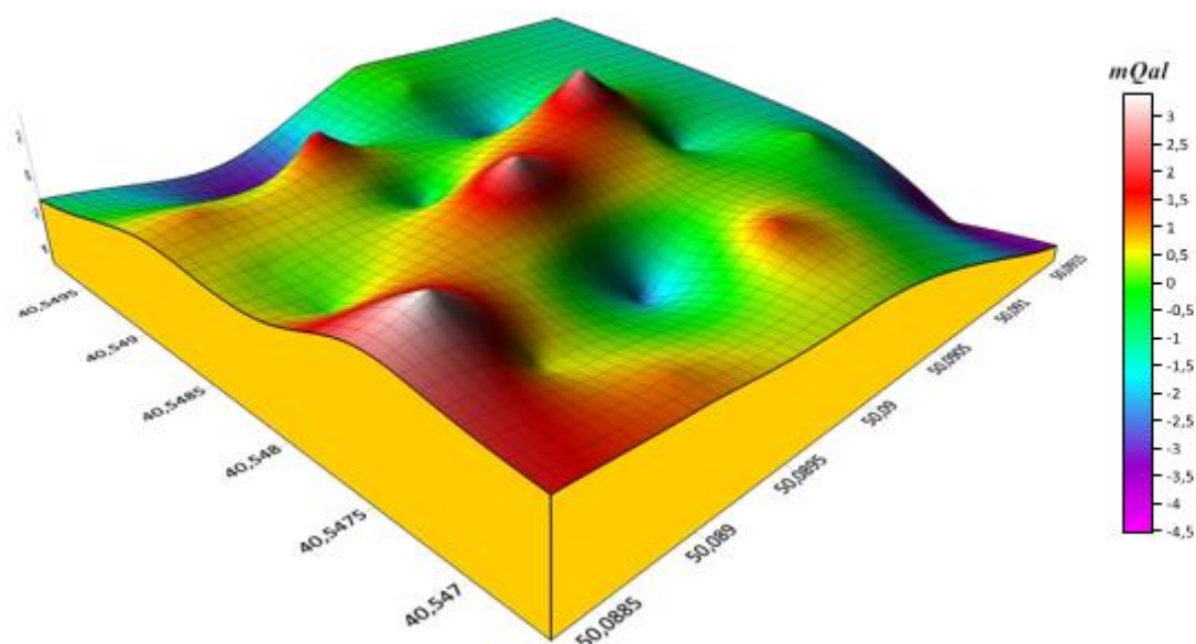
Fig. 6. 3D model reflecting the stress-strain state of the study area
