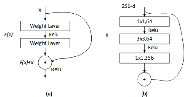
Figure 2. ResNet architectures. (a) Basic residual block, (b) Residual block used for ResNet110.
