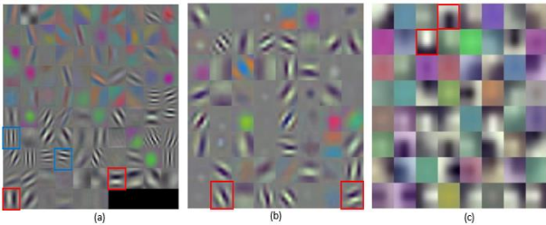
Figure 3. Hidden layer weight visualization (a) AlexNet, (b) ResNet50, (c) VGG16.
