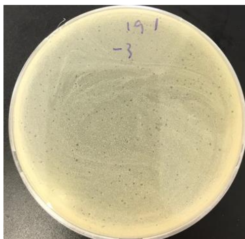
Figure 1. Appearance of clear plaque formed by SA-19 phage with its host with the double layer agar method.
