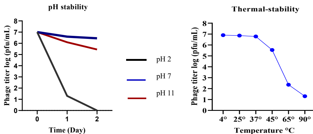
Figure 2. pH and thermal stability on phage SA-19.
