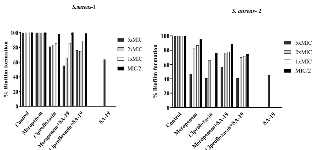
Figure 5. Eradication of mature biofilm biomass of S. aureus strains by antibiotics (5×MIC, 2×MIC, 1×MIC, MIC/2) and phages alone or in combination.
