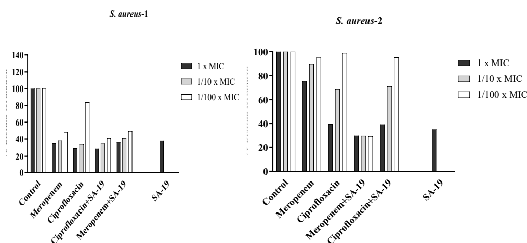
Figure 4. Inhibition of biofilm formation of S. aureus strains by antibiotics and phage SA-19 alone or in combination.
