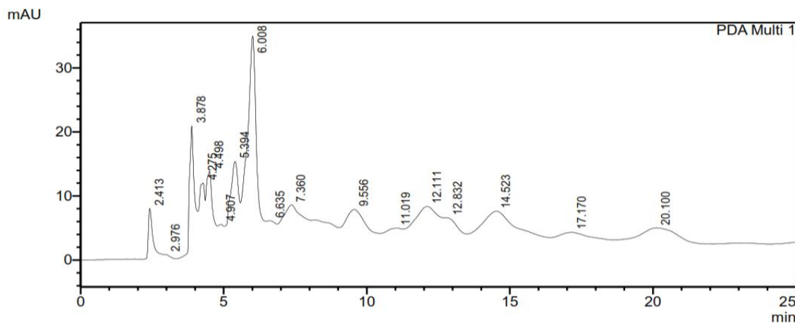
Figure 1. HPLC profile of F8. The analysis using Shimadzu HPLC system, Lichrospher RP-18 column (4.6 × 250 mm, 5 μm), gradient mobile phase acetonitrile-water 50%-50% to 80%-20%, flowrate 0.5 mL/min and observed at 254 nm.
