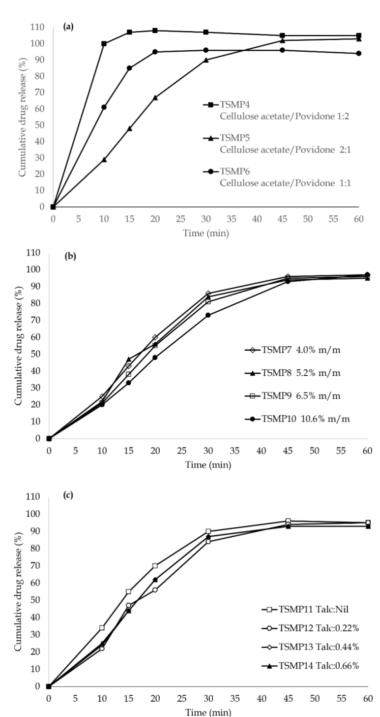
Figure 5. Effect of different formulation variables on the dissolution of topiramate from different batches of taste masked MUPS. (a) effect of ratio of cellulose acetate-povidone on dissolution; (b) effect of concentration of taste masking polymer concentration (in terms of weight gain) on dissolution; (c) effect of concentration of talc on dissolution.
