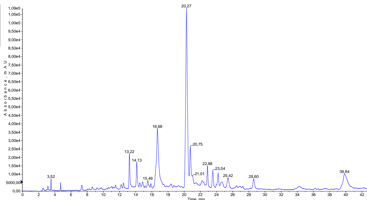
Figure 1. HPLC-MS/MS chromatogram of 70% MeOH extract of I. oculus-christi .
