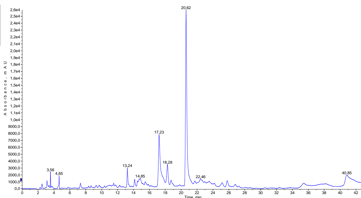
Figure 2. HPLC-MS/MS chromatogram of 5% infusion of I. oculus-christi .
