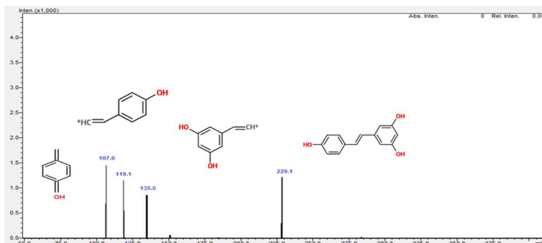
Figure 4. The main ion and fission ions of RES
