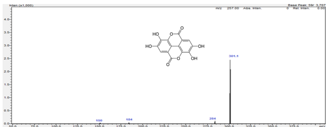
Figure 3. The main ion and fission ions of EA
