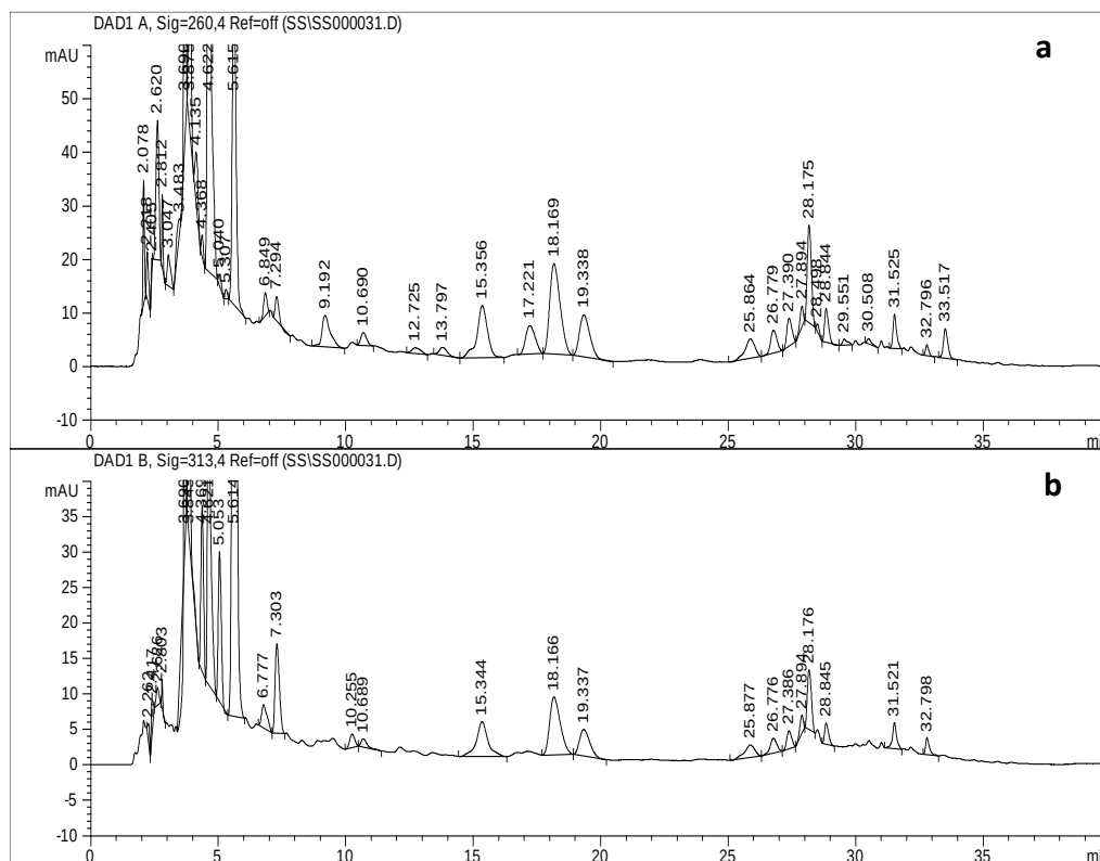
Figure 1. Chromatogram of the blueberry sample. Rt(EA): 17.22, Rt(RES): 32.79 (a. \lambda=260 nm, b. \lambda=313 nm)
