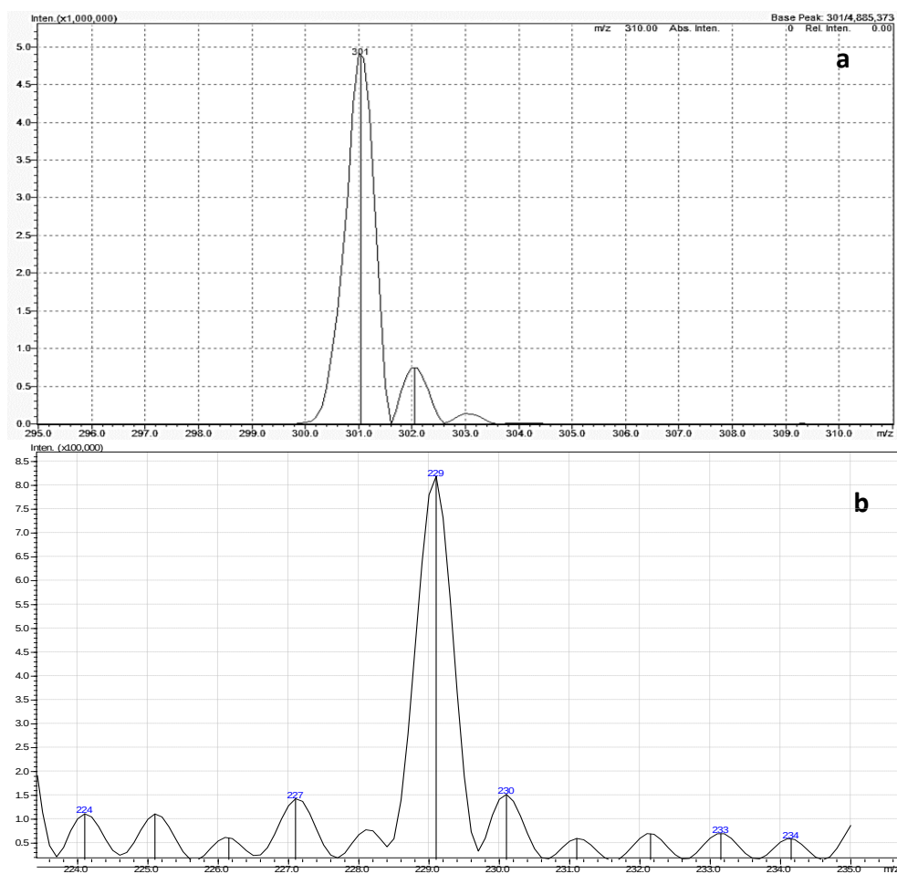
Figure 2. a) [M+H]^+ = 229.1 m/z in positive polarity molecular ion spectrum of RES, b) [M+H]^+ = 229.1 m/z molecular ion chromatogram of RES.
