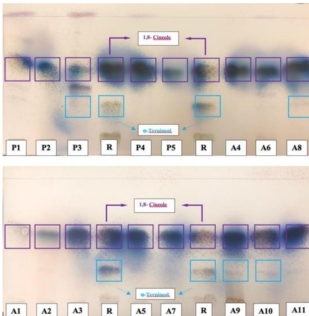
Figure 2. TLC chromatogram of all samples. R: Reference mixture; 1,8-cineole and α-terpineol from top to bottom. Mobile phase; ethyl acetate:toluene (10:90 V/V). Detection: sprayed with anisaldehyde solution R and heated at 100-105 °C for 5-10 min; examined in daylight.
