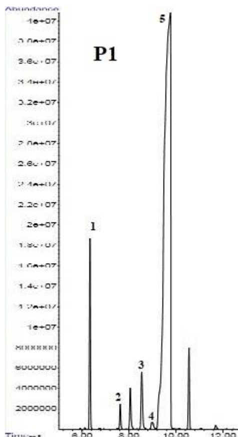
Figure 3. GC-MS chromatogram of P1 sample showing the chemical components given in pharmacopoeia: 1: \alpha -pinene, 2: \beta -pinene, 3: \alpha -phellandrene, 4: limonene and 5: 1,8-cineole
