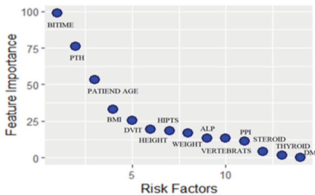
Figure 2. Feature importances based on RF
