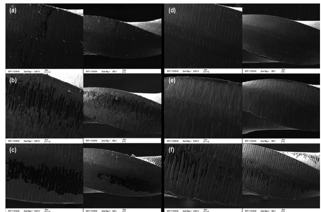
Figure 2. File images after preparation (original magnifications \times 500 and \times 1,000 ). (a) group 3-F1 file, (b) group 2-F1 file, (c) group 1-F1 file, (d) group 3-F2 file, (e) group 2-F2 file and (f) group 1-F2 file
