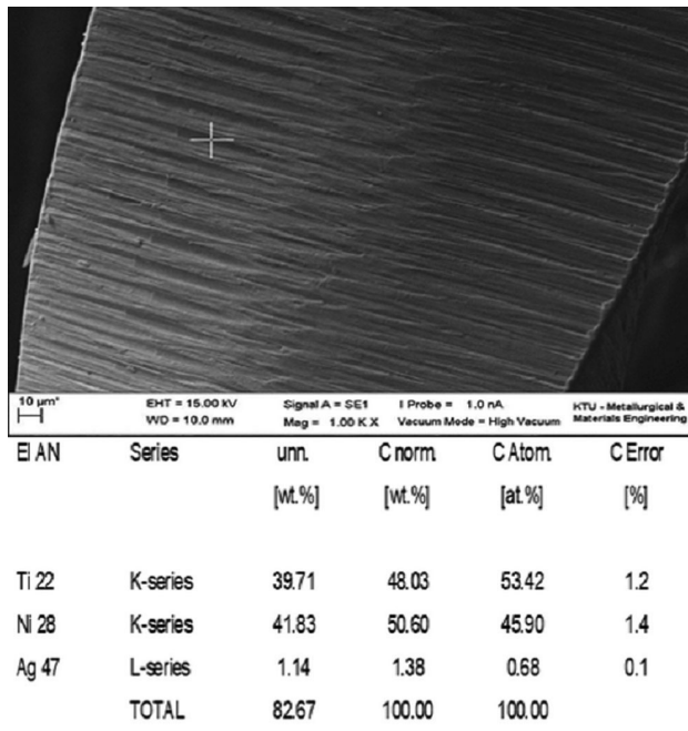
Figure 4. Ni, Ti and Ag were detected with an elemental analysis performed in regions with a different shade in the coated groups after preparation
