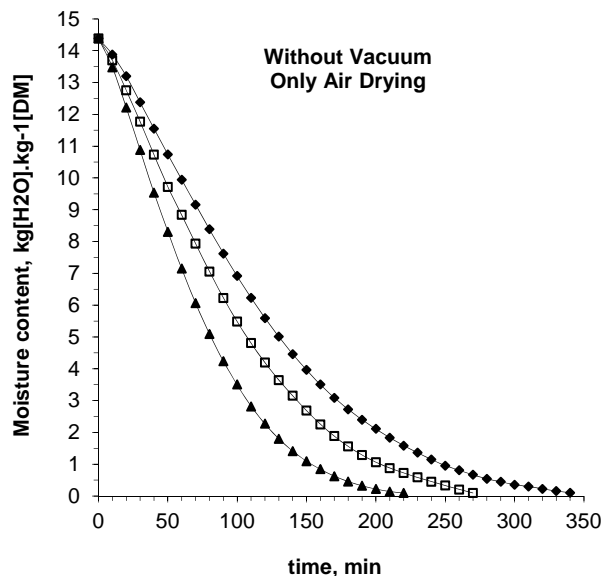
Figure 3. The air drying curve of celeriac slices on dry basis (kg[H 2 O].kg -1 [DM]); ▲, 75°C; □, 65°C; ◆, 55°C.
