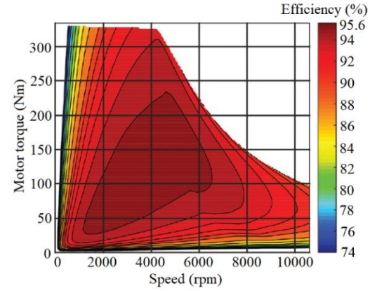
Figure 4. Electric motor speed, torque, and efficiency map
