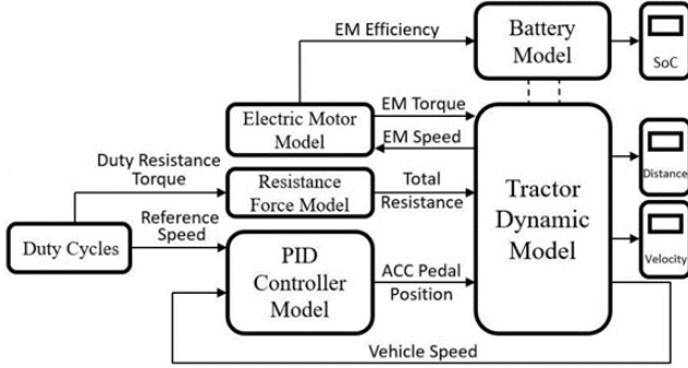
Figure 1. Schematic representation of electric tractor systems
