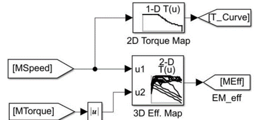
Figure 5. Electric motor Simulink model
