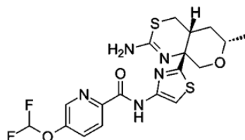
Figure 63. Molecular structure of PF-06751979
