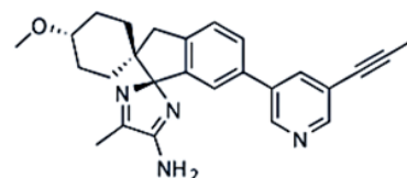
Figure 58. Molecular structure of LY3314814
