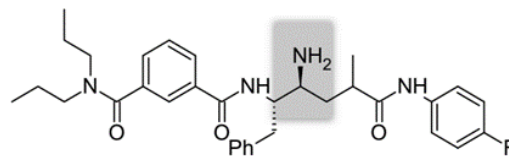
Figure 19. Compound 22. IC_{50} = 26 \mu M [33]
