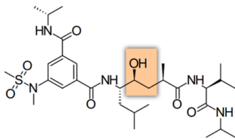
Figure 10. Compound 10. IC_{50} = 39 \mu M [38]
