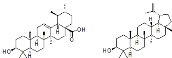
Figure 44. The chemical formulas of ursolic acid and lupeol
