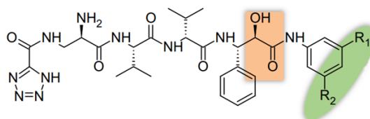
Figure 7. Compound 4 R_1 and R_2 = Tetrazole, IC_{50} = 1.2\ \mu\text{M} . Compound 5 R_1 and R_2 = Cl, IC_{50} = 14\ \mu\text{M} [34]
