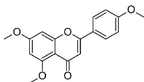
Figure 43. 5,7,4'-Trimethoxyflavone (TMF) IC_{50} = 0.569 nM [69]
