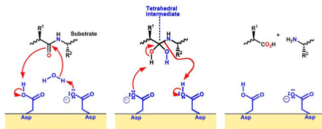
Figure 3 Mechanism of action of catalytic aspartic acid residues [31]
