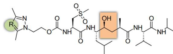
Figure 9. Compound 8. IC_{50} = 0.3\ \mu\text{M} . R = \text{C} . Compound 9. IC_{50} = 0.12\ \mu\text{M} . R = \text{O} [37]
