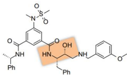
Figure 17. Compound 19. IC_{50} = 10 \mu M [41]
