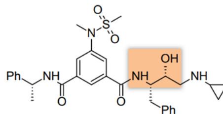
Figure 13. Compound 12. IC_{50} = 15 \mu M [34]
