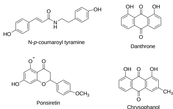
Figure 51. The molecular structure of N-p-coumaroyl thyramine, danthrone, ponsiretin, and chrysophanol
