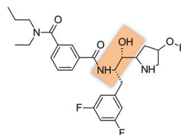
Figure 15. Compound 14. IC_{50} = 5 \mu M. R = -Benzyl. Compound 15. IC_{50} = 3 \mu M. R = - Phenyl. Compound 16. IC_{50} = 8 \mu M. R = (-Et) 2 [30]
