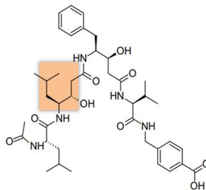
Figure 4. Compound 1. IC 50 = 21 \mu M [30]
