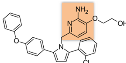
Figure 25. Compound 31 [20]
