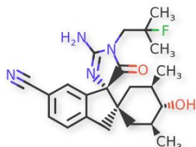
Figure 56. Molecular structure of BI 1181181
