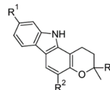
Figure 48. Compound 60. IC_{50} = 0.017 nM [78]
