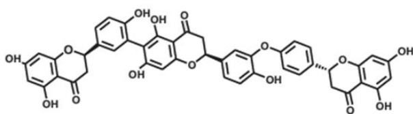
Figure 50. Compound 61. IC_{50} = 0.75 \mu M [82]
