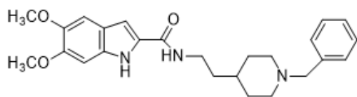
Figure 39. Compound 52 IC_{50} = 0.39 \mu M [6]
