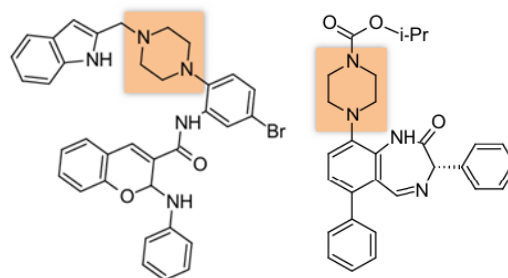
Figure 34. Compound 44. IC_{50} = 0.08 nM. Bileşik 45. IC_{50} = 0.289 nM [41]
