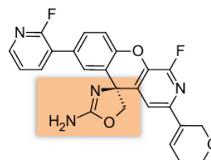
Figure 31. Compound 39. IC 50 = 0.3 nM [54]
