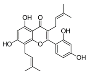
Figure 45. Compound 57. IC_{50} = 0.034 nM [73]
