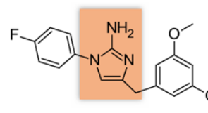
Figure 26. Compound 32. IC_{50} = 740 nM [45]
