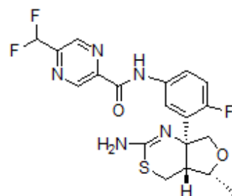
Figure 60. Molecular structure of E2609
