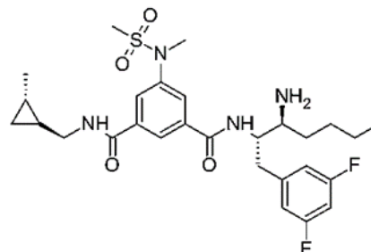
Figure 20. Compound 23. IC_{50} = 90 \mu M [41]
