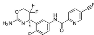
Figure 55. Molecular structure of RG7129
