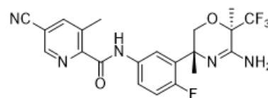
Figure 42. Compound 56. IC_{50} = 5 \mu M [66]
