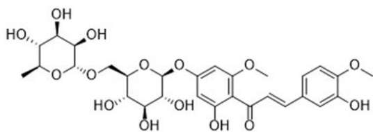
Figure 52. The chemical structure of compound 62
