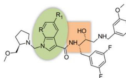
Figure 16. Compound 17. IC_{50} = 18 \mu M. R = -C, R1 = -CN. Compound 18. IC_{50} = 20 \mu M. R = -N, R1 = -CH 3 [33]
