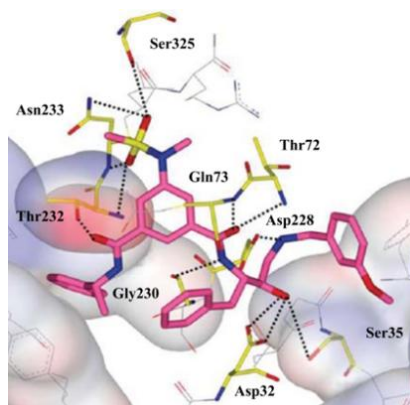
Figure 12. X-ray crystalline structure of the inhibitor-enzyme complex for compound 18 [41]
