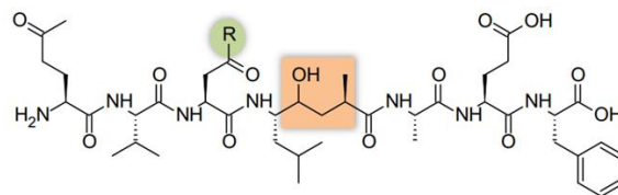
Figure 8. Compound 6 (OM99-2). IC_{50} = 1.6\ \mu\text{M} . R = -\text{NH}_2 . Compound 7 (OM99-3). IC_{50} = 0.3\ \mu\text{M} . R = -\text{OH} [35]
