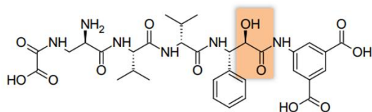
Figure 6. Compound 3. IC_{50} = 0.20\ \mu\text{M} [33]
