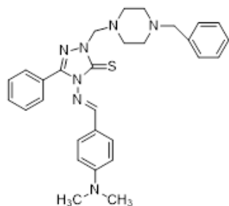
Figure 38. Compound 51 IC_{50} = 0.709 \mu M [63]
