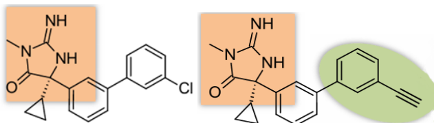
Figure 28. Compound 35. IC 50 = 21 nM [48] Compound 36. IC 50 = 5.4 nM [49]
