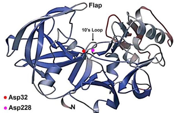
Figure 1 Three important components of the BACE-1 enzyme: catalytic aspartic acid residues, wing and 10-second cycle point [26]
