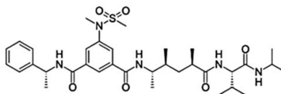
Figure 64. The molecular structure of CTS21166
