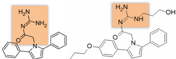
Figure 22. Compound 25. IC_{50} = 370 nM. Compound 26. IC_{50} = 110 nM [38, 43]
