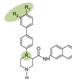
Figure 35. Compound 46. IC_{50} = 0.03 nM. R=-C, R 1 =-H, R 2 =-H. Bileşik 47. IC_{50} = 0.023 nM. R=-N, R 1 =-F, R 2 =-Cl [30]
