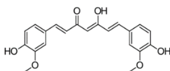
Figure 46. Compound 58. IC_{50} = 0.025 nM [74, 76]
