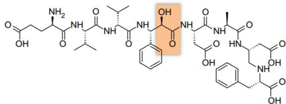
Figure 5. Compound 2. IC_{50} = 50\ \mu\text{M} [33].
