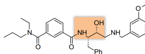
Figure 14. Compound 13. IC_{50} = 20 \mu M [34]
