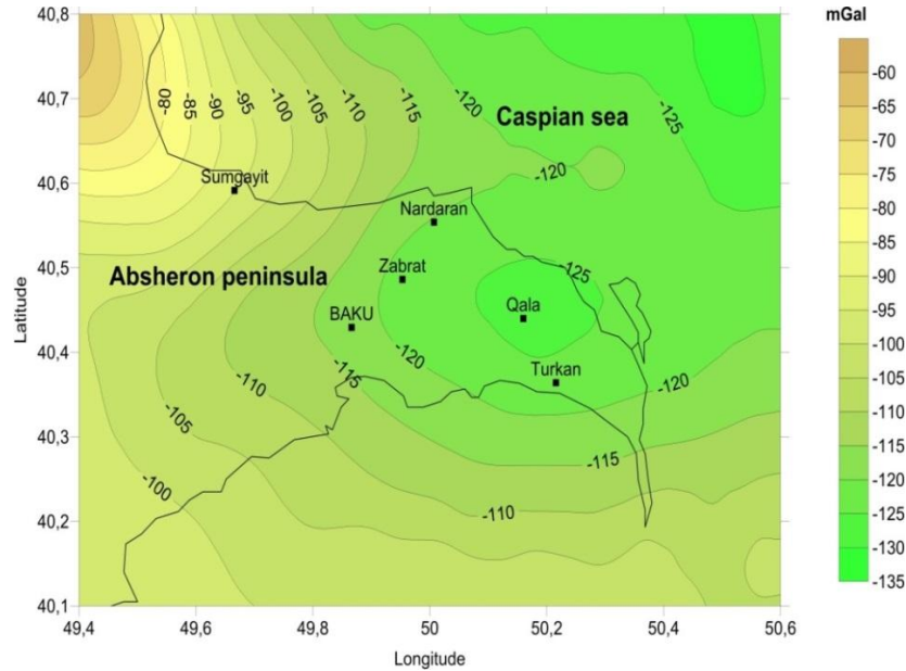
Figure 1. Bouguer gravity map of the Absheron Peninsula
