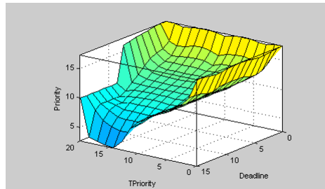
FIGURE 3. The decision surface corresponding to Inference rules
