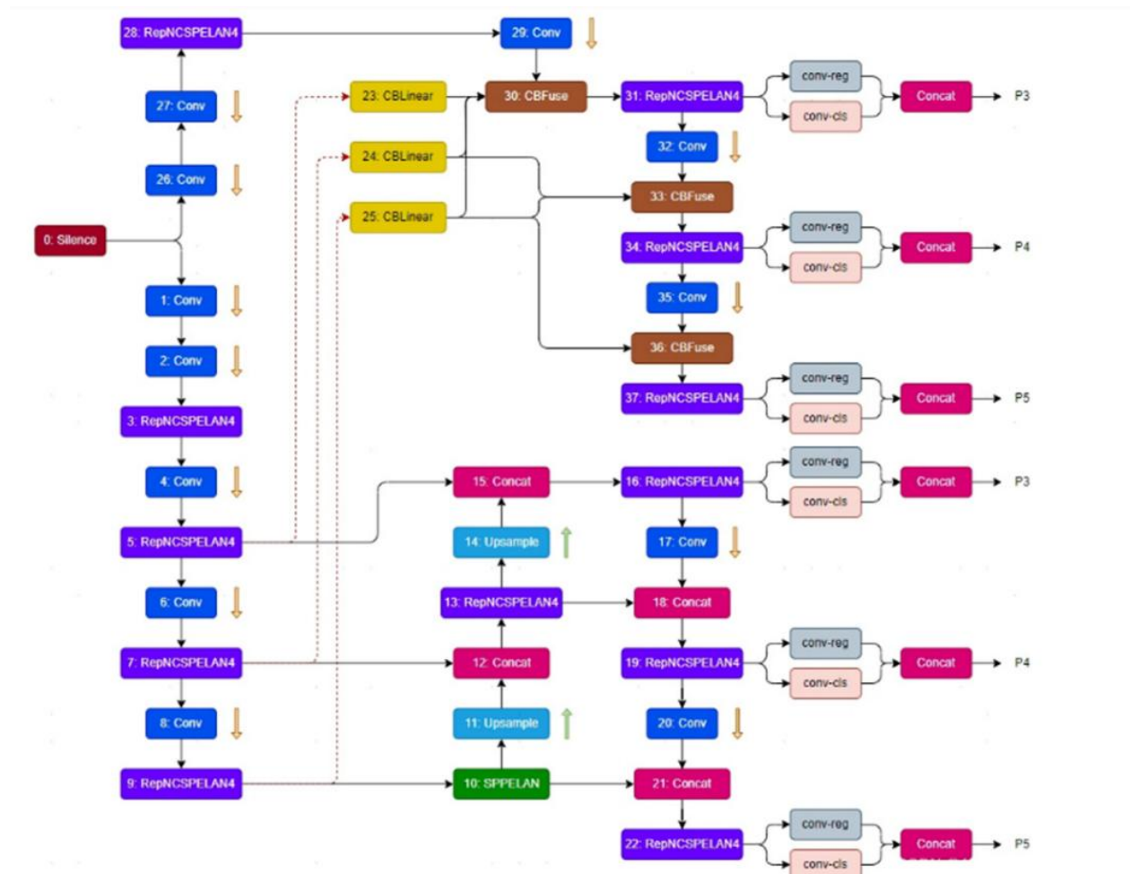
Figure 3: YOLOv9 architecture (Wang, 2024)
