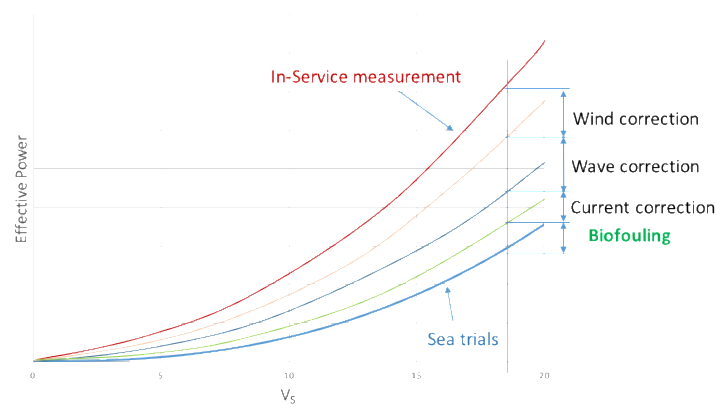
Fig. 22. Schematic representation of deterministic corrections for external disturbances
