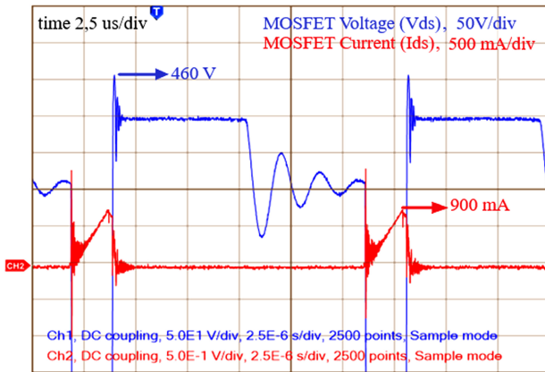
Fig. 7. The voltage and the current waveforms of the MOSFET.
