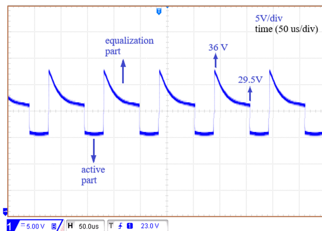
Fig. 10. The data transfer signal in KNX with choke.
