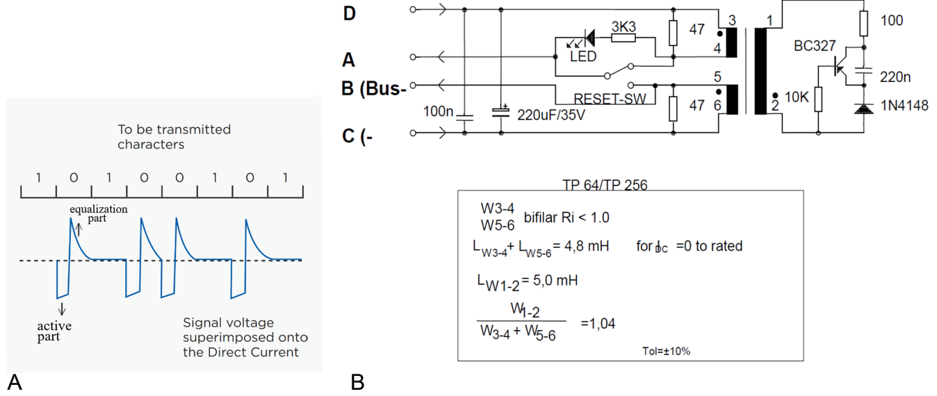
Fig. 5. (a) Signal shape in KNX system. (b) Electrical circuit of a choke module.
