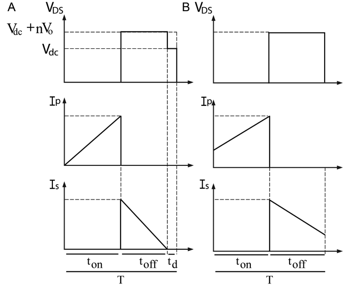
Fig. 2. Typical flyback converter. (a) DCM operation. (b) CCM operation [10].
