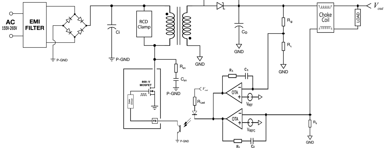
Fig. 3. Flyback converter circuit scheme designed for KNX standards.
