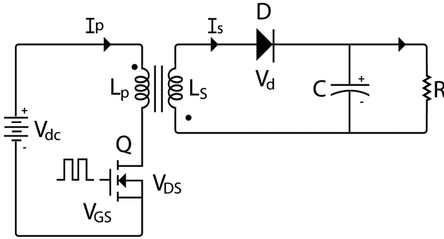
Fig. 1. The conventional flyback converter scheme [10].
