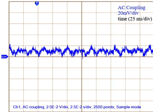
Fig. 9. The ripple waveform of the output voltage.
