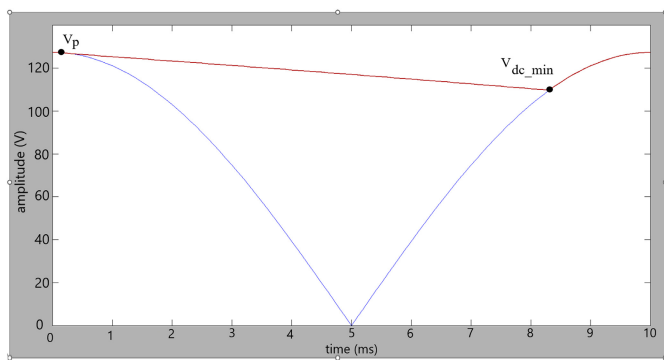
Fig. 4. V_{dc} voltage waveform simulation results.
