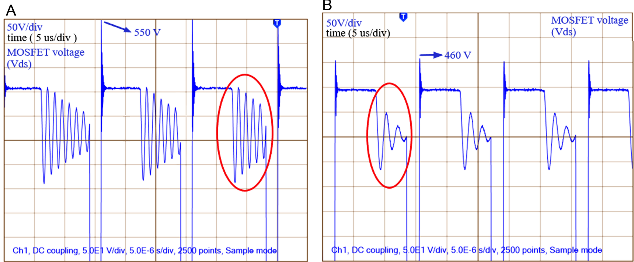
Fig. 6. The voltage stresses of the MOSFET for 220 V RMS: (a) without snubber cell and (b) with snubber cell.
