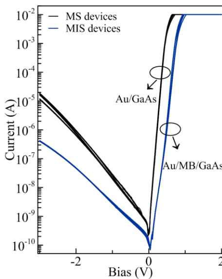
Figure 5. I-V characteristics of Au/GaAs and Au/MB/GaAs devices, at room temperature and in the dark.
