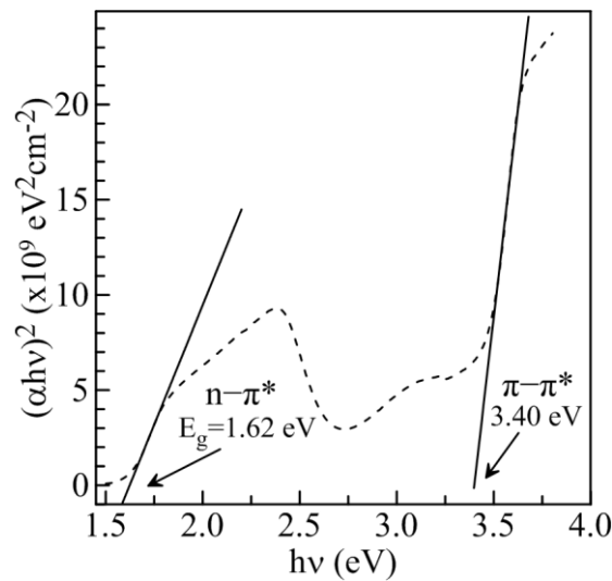
Figure 2. (\alpha hv)^2 vs. h\nu graphs of the MB.
