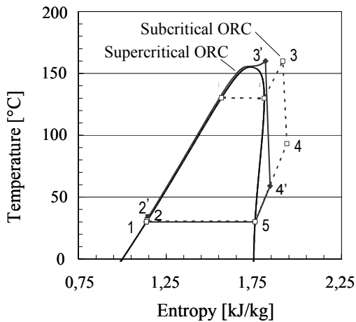
Figure 2. Sub- and supercritical ORC. Example of R245fa.
