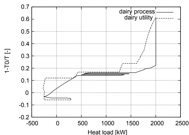
Figure 14. Integrated composite curves for optimized refrigeration cycle.
