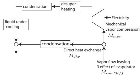
Figure 12. MVR integration.
