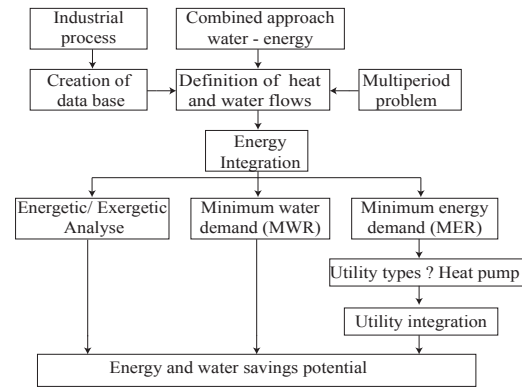
Figure 3. Heat pump integration methodology.
