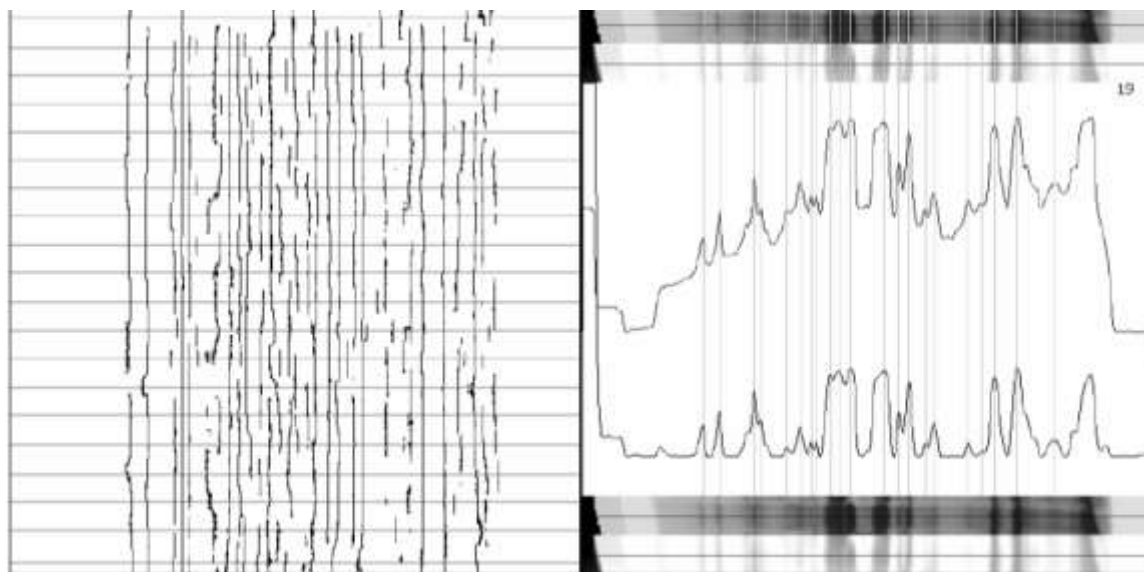
Figure 4. a) The local minima in the image corresponding to bands above the noise threshold; b)
