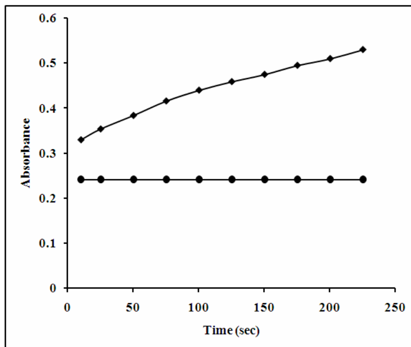
Figure 1. Absorbance-time curve for ( ) 0.29 \mu\text{g mL}^{-1} Ni(II) and ( ) 0.183 \mu\text{g mL}^{-1} Mn(II). The absorbances recorded at wavelength 565 nm in fixed time (10-200 s).
