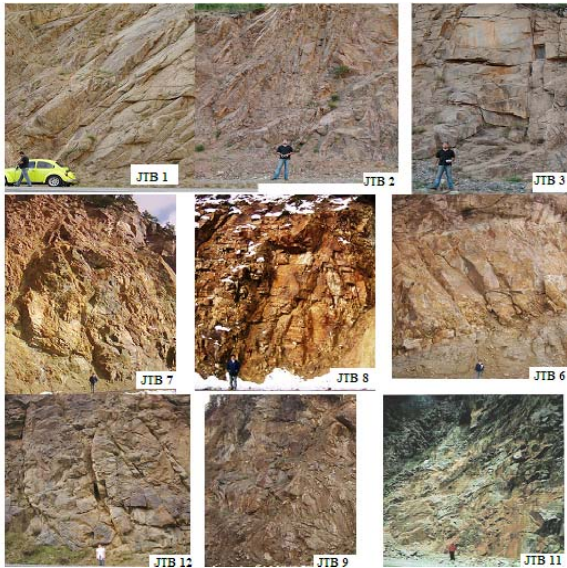
Figure 4. Geotechnical units (JTB) determined in magmatic rocks exposed in the selected slope.
