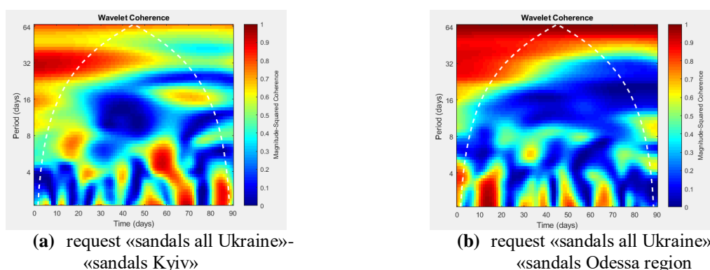
Figure 3. Wavelet coherence between data rows that reflect the level of interest in the sandals by region of Ukraine.
