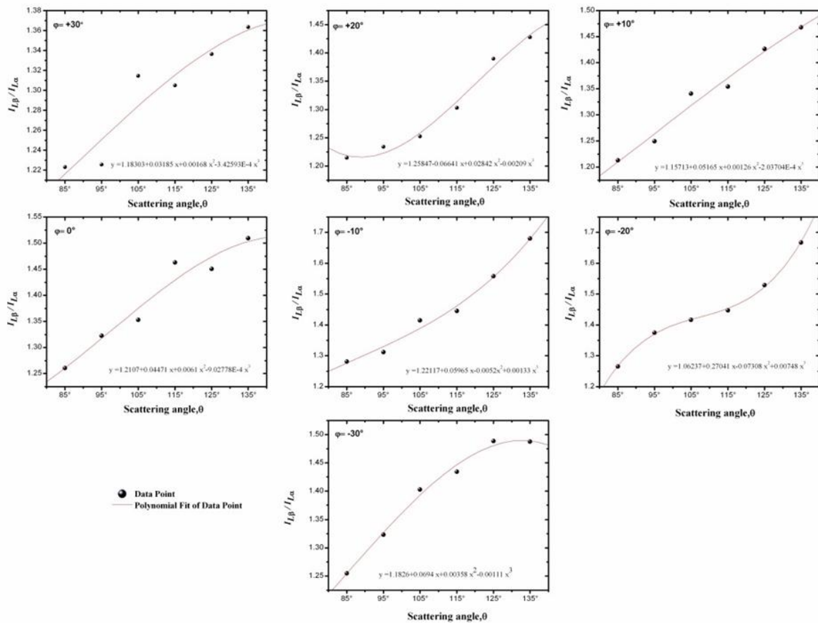
Figure 4. The variation of L_\beta / L_\alpha with the scattering polar angles ( \theta ) at a fixed azimuthal scattering angle.
