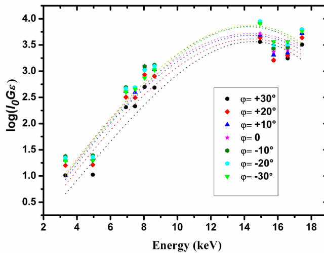
Figure 3. The efficiency graph of the detector for the polar scattering angle ( \theta = 115^\circ ).
