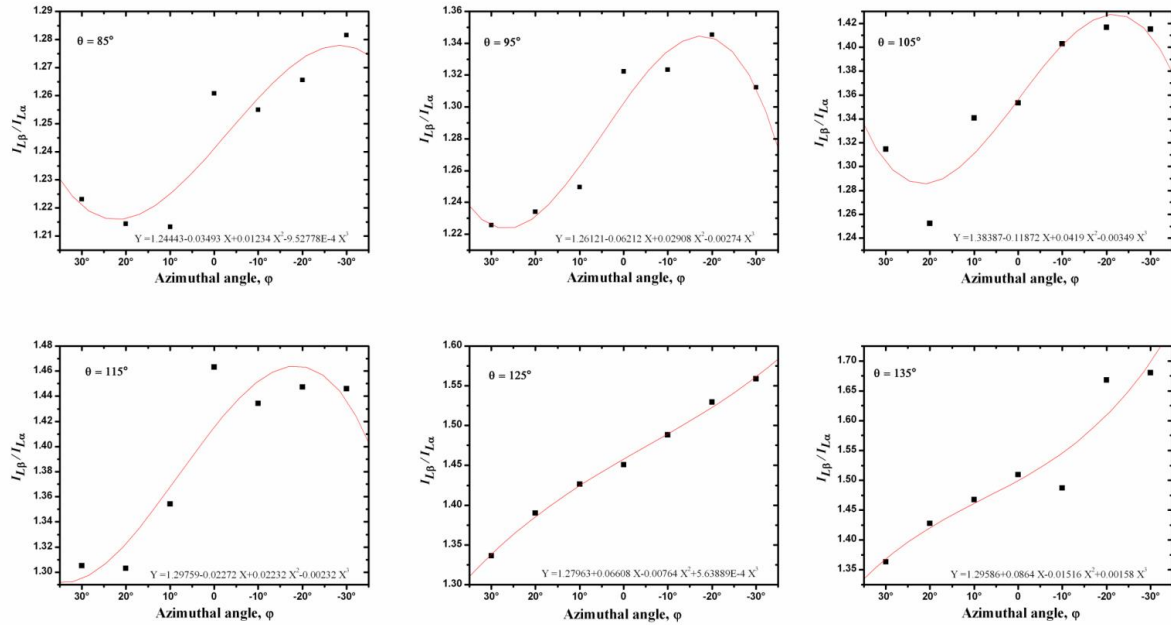
Figure 5. The variation of L_{\beta}/L_{\alpha} with the azimuthal scattering angles ( \varphi ) at a fixed scattering polar angle.
