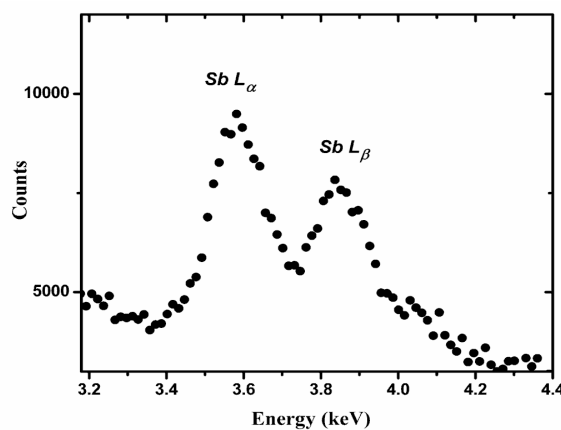
Figure 2. Typical spectrum for L_{\alpha} and L_{\beta} rays of Sb.
