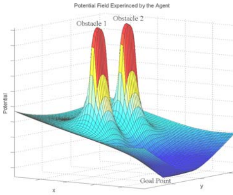
Figure 4. Potential field created by two obstacles and a goal point.
