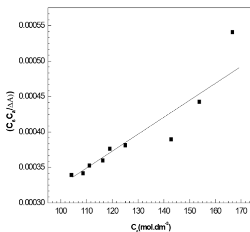
Figure 3c. Plot for calculation of binding constant ( K_{\alpha\beta} ) for CV/SDS system.
