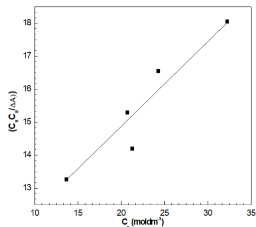
Figure 5b. Plot for calculation of binding constant ( K_{a\beta} ) for CV/SDS system.
