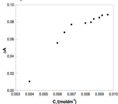
Figure 3a. Plot of differential absorbance of CV as a function of SDS concentrations.
