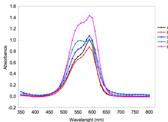
Figure 2a. Absorption spectral of 1.0 \times 10^{-5} moldm -3 CV at various concentrations of SDS at 298.15K. Concentrations of SDS (moldm -3 ): (A) 2.0 \times 10^{-4} ; (B) 4.0 \times 10^{-4} ; (C) 2.0 \times 10^{-2} ; (D) 4.0 \times 10^{-2} and (E) 0.00.
