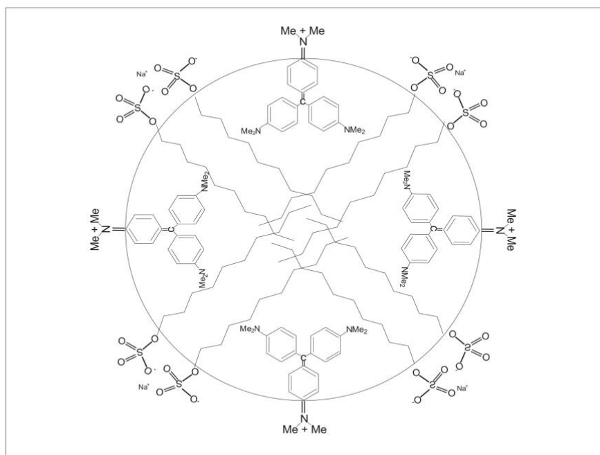
Figure 6b. Proposed locus of CV in SLS micelle.
