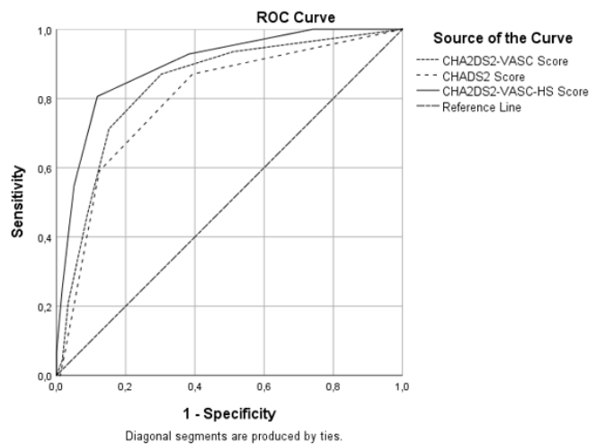
Figure 2. Receiver operating characteristic (ROC) curve with calculated area under the curve and optimal cut-off point for the CHA2DS2VASC score, CHADS2 score and CHA2DS2VASC-HS score to identify the presence of STR failure. C-Statistic (area under the curve) — 95% confidence interval (95% CI): CHADS2: 0.797 (0.793-0.884), P < 0.001 ; CHA2DS2-VASc: 0.839 (0.747-.0.848), P < 0.001 ; CHA2DS2VASC-HS: 0.896 (0.861-.0.931), P < 0.001 . We calculated that a cut-off point of 1.5 for CHA2DS2-VASc score, 0.5 for CHADS2 and 3.5 for CHA2DS2-VASc-HS score could estimate the presence of STR failure with a sensitivity of 87 %, 87 % and 80 % ; a specificity of 70 %, 60 %, 88 % respectively.
