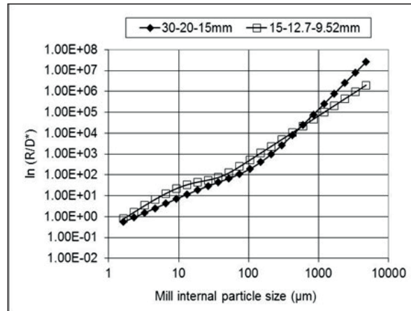
Figure 8. Specific breakage rate parameter in industrial scale two stage open circuit grinding case at different grinding media applications
