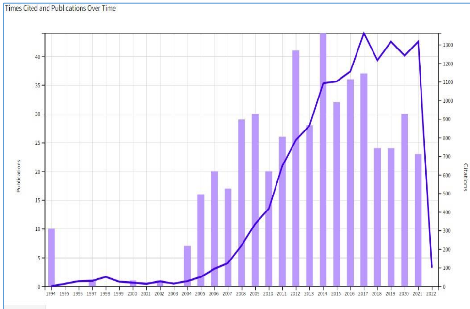
Graph 1: Times Cited and Publications Dealing With Obesity Over 1994-2022.
