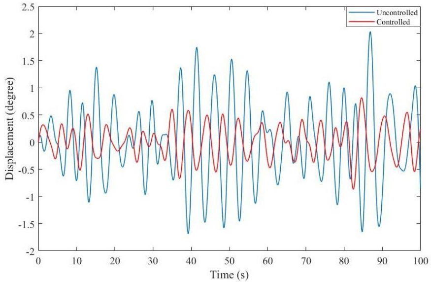
Figure 13: Comparison of Uncontrolled and PID-controlled Responses of the Pitch Motion
