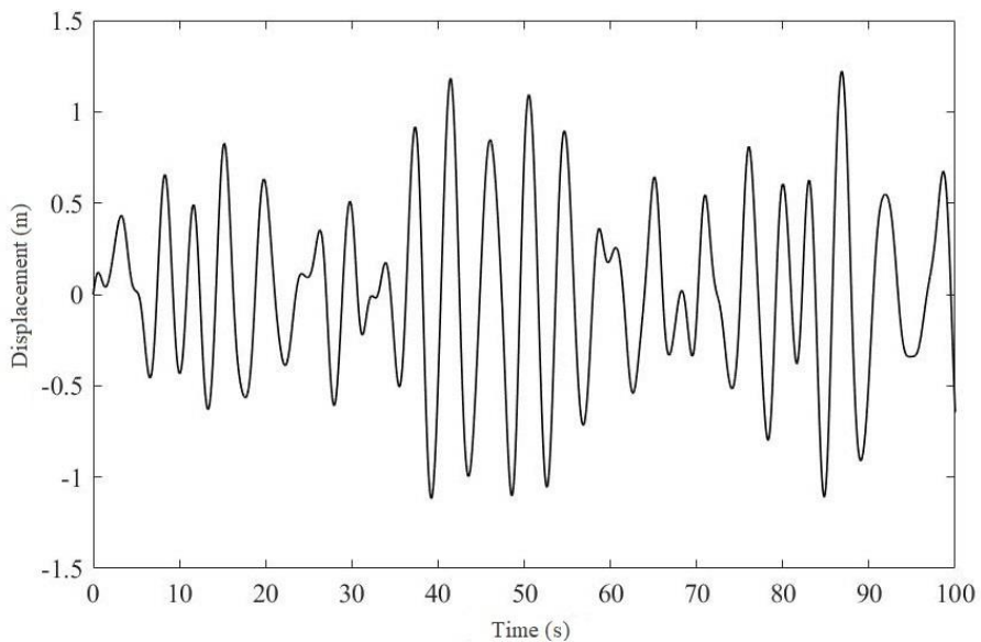
Figure 6: Change of Heave Motion Under Random Head Waves
