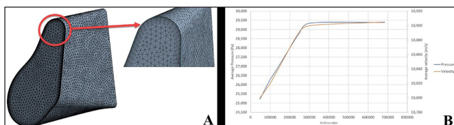
Figure 4. A. Mesh structure for NVR model. B. Grid independence test.
