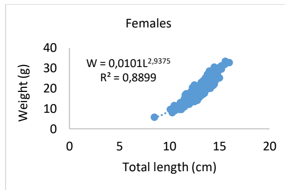
Figure 3. The length–weight relationships (LWRs) females of horse mackerel Trachurus trachurus (Linnaeus, 1758) in the Sea of Marmara
