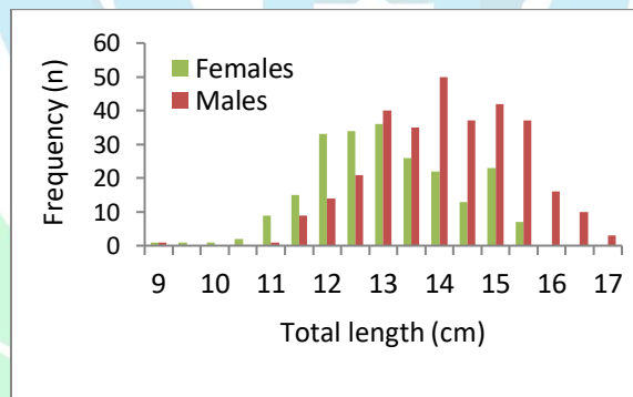
Figure 2. Length frequency distribution of males and female samples of the horse mackerel Trachurus trachurus (Linnaeus, 1758) in the Sea of Marmara
