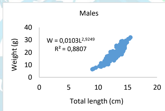
Figure 4. The length–weight relationships (LWRs) males of horse mackerel Trachurus trachurus (Linnaeus, 1758) in the Sea of Marmara
