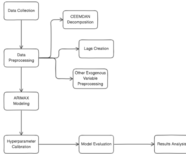
Figure 4. Methodology Workflow
