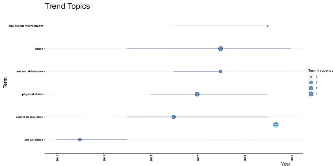
Figure 8. Trend Topics
