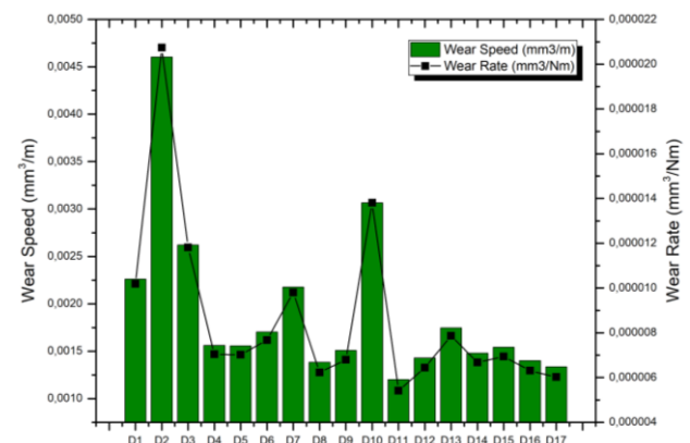
Figure 7. Wear rate and speed of the samples.
