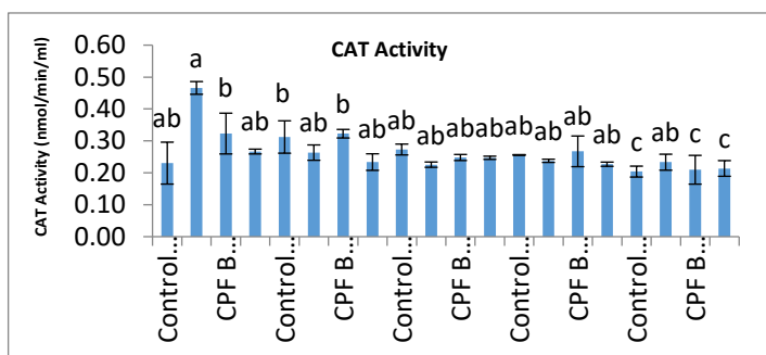
Figure 2d. CAT enzyme activity values of CPF pesticide active ingredient on N. cryptocephala var. veneta . Different letters on the bar indicate statistical differences p < 0.05 according to experimental groups. Values represent the mean \pm SE
