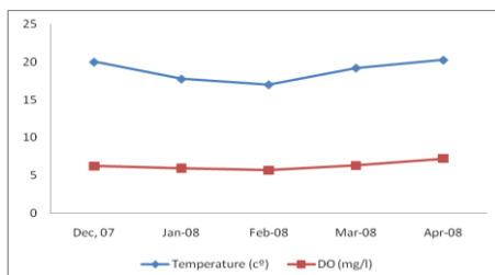
Figure 1. Average temperature and Dissolved oxygen levels for surface waters
