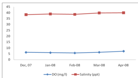
Figure 2. Dissolved oxygen levels versus salinity on surface waters
