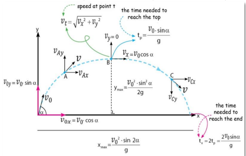
Figure 8. Parabolic Motion Track
