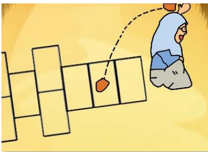
Figure 7. When Gaco is Thrown into a Game Plot and Forms a Quarter Circle or Half Parabolic Motion
