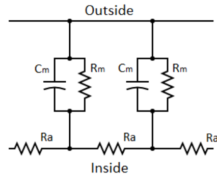
Fig.1. Electrical Modeling of Passive Membrane
