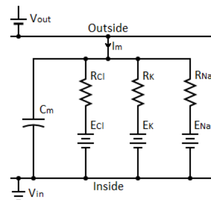
Fig.2. Electrical Modeling of Passive Membrane with Different Ion Channels
