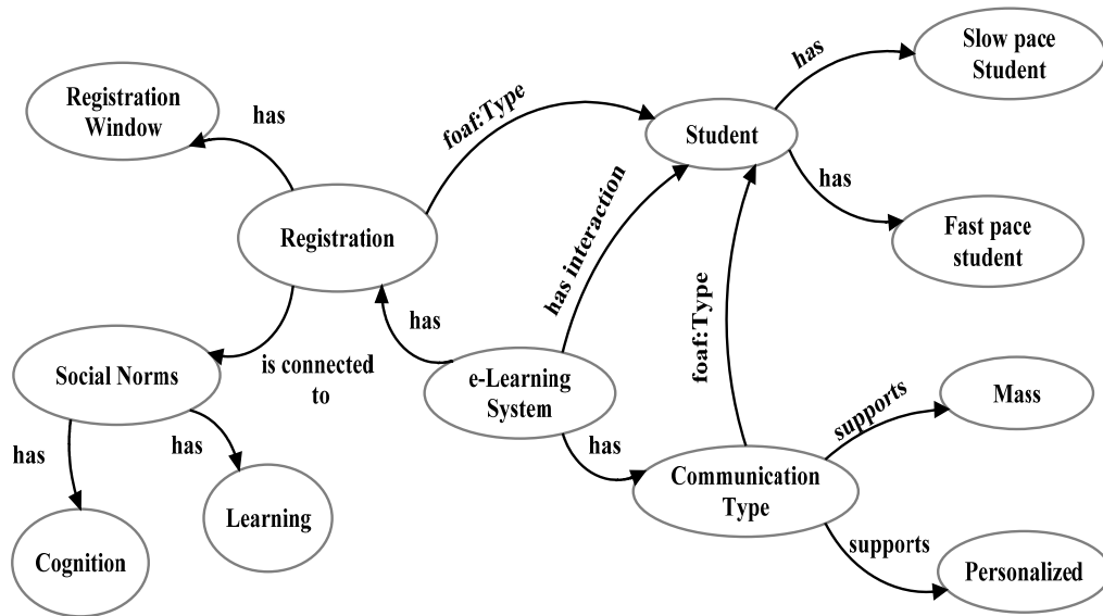
Figure 5: Ontology framework of e-Learning Norms
