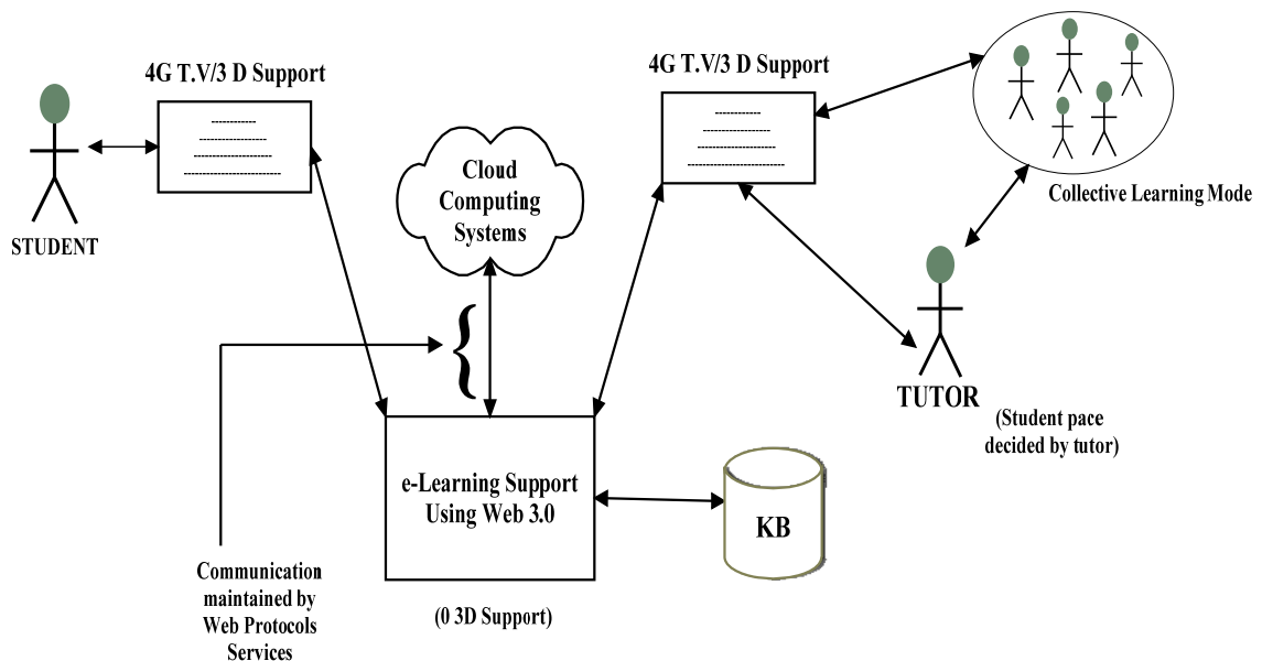
Figure 6: Web 3.0 support to e-Learning using 4 G T.V with 3-D
