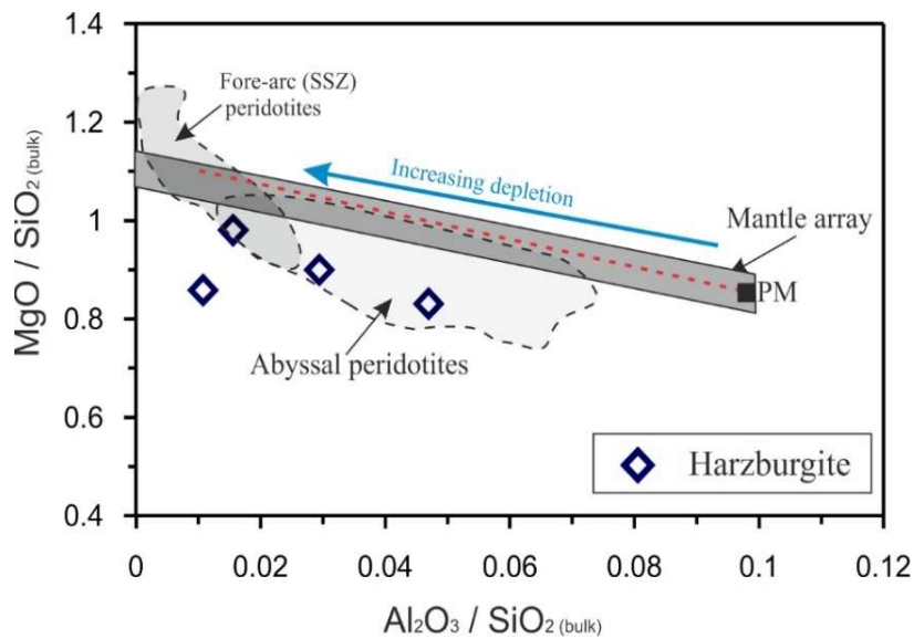
Fig. 7. Whole rock major element distribution of harzburgites in MgO/SiO 2 and Al 2 O 3 /SiO 2 exchange diagram (after Wu et al. (2017))
